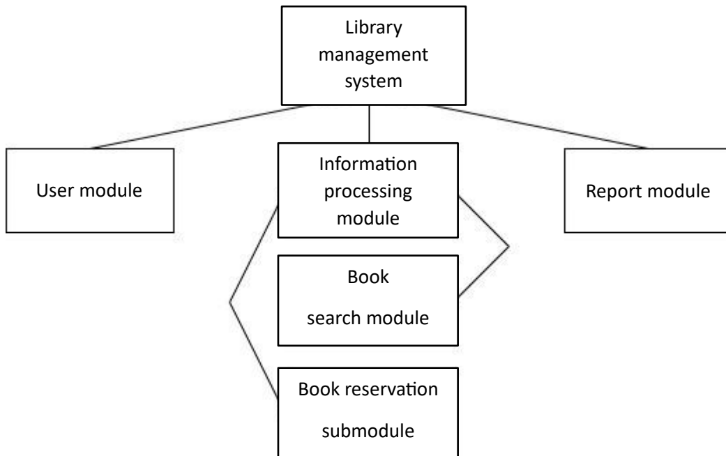
Image 1 – Modular Decomposition
