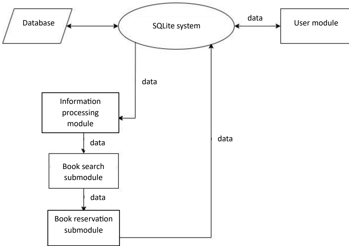
Image 2 - Inter-module dependencies
