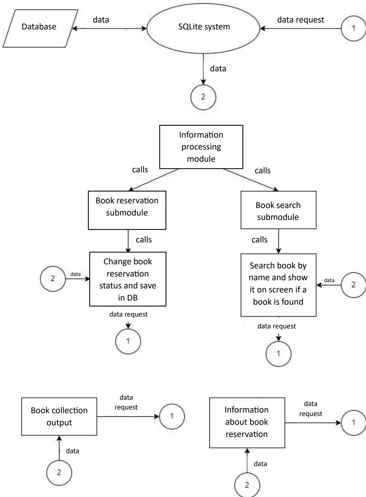
Image 3 - Inter-process dependencies
